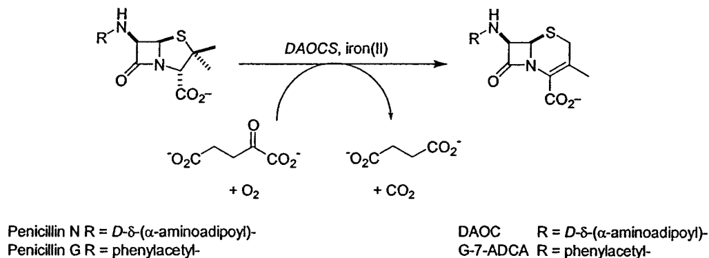
SCHEME 1. The ring expansion reaction catalyzed by DAOCS. G-7-ADCA, phenylacetyl-7-aminodeacetoxycephalosporanic acid.
